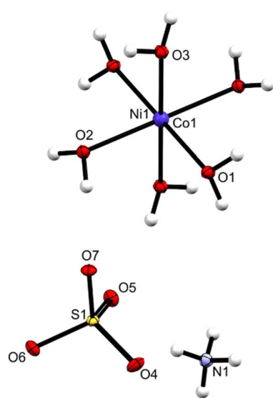
Fig. 1 (Left) View of the [\text{Ni}_{0.78}/\text{Co}_{0.22}(\text{H}_2\text{O})_6]^{2+} , \text{SO}_4^{2-} and \text{NH}_4^+ cation in 1 . The central atom in the complex cation is labeled as both Ni and Co atoms as the site is shared by the two atoms. The thermal ellipsoids are drawn at 50% probability. The three symmetrically equivalent O atoms and all H atoms are unlabeled and (Right) isolated Tutton's salt crystals.
