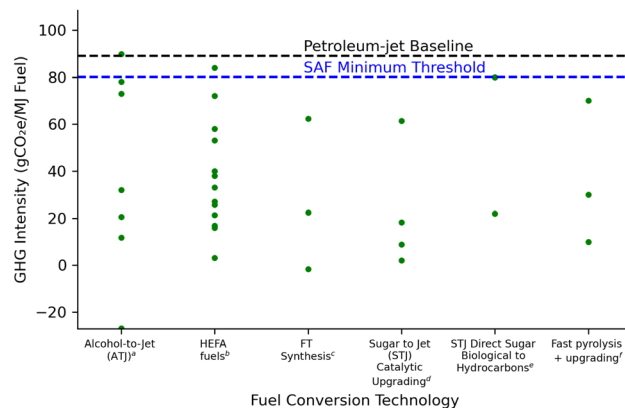
Fig. 1 GHG intensity SAF pathway comparison to fuel conversion technology pathways: ATJ, HEFA fuels, FT synthesis, and STJ catalytic. a Han (2017), 37 Gollakota (2021), 39 Staples (2014), 33 Budsberg (2016), 34 Tanzil (2022). 40 b Cox (2014), 38 Stratton (2011), 41 de Jong (2017), 42 Bailis (2010), 15 Seber (2014). 43 c Shonnard (2010), 44 de Jong (2017), 42 Suresh (2018). 29 d Riazzi (2018), 35 Baral (2021). 36 e Han (2017), 37 Cox (2014). 38 f Sorunmu (2017), 30 Elkasabi (2020), 45 Fitriarsari (2023). 31
