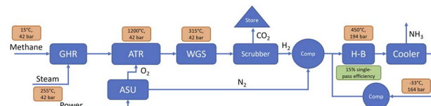
Fig. 3 Simplified process drawing of the ATR-based blue ammonia synthesis process. "GHR" is the gas heated reformer, "ATR" the autothermal reformer, "WGS" is the water gas shift reactor, "H–B" the Haber–Bosch reactor, "ASU" the air separation unit, and "Comp" are compressors.
