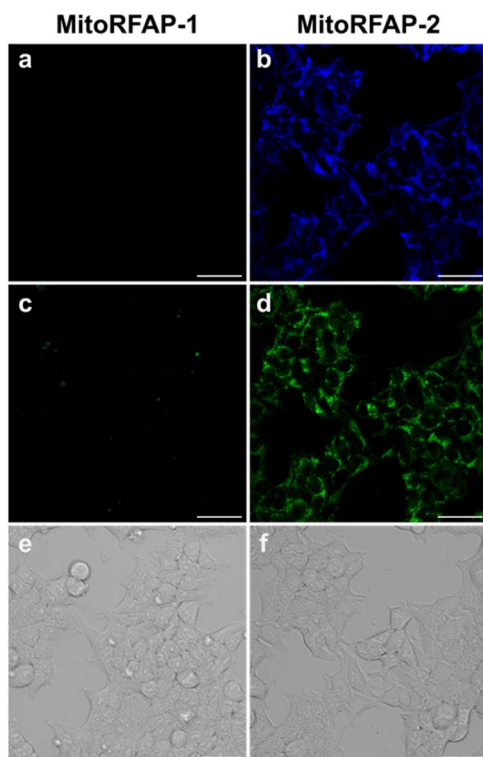
Fig. 2 Live HEK 293T cells stained with (a) MitoRFAP-1 (2 \mu\text{M} ) or (b) MitoRFAP-2 (2 \mu\text{M} ) imaged with \lambda_{\text{ex}} = 405 \text{ nm} and the (c and d) respective \lambda_{\text{ex}} = 488 \text{ nm} images and (e and f) respective brightfield images. The data show the superior cell-permeability of MitoRFAP-2. Scale bar represents 40 \mu\text{m} in all images.
