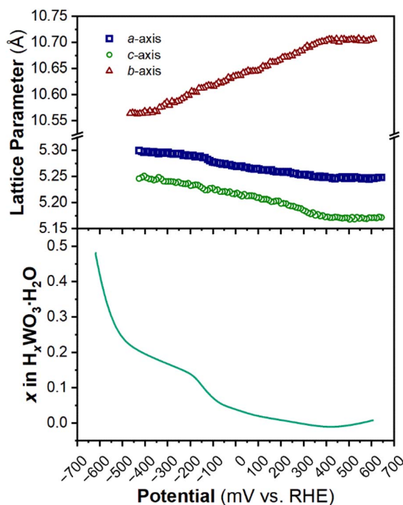
Fig. 9 Trend of lattice parameters (from Pawley refinements of the operando XRD) and proton composition in \text{H}_x\text{WO}_3 \cdot \text{H}_2\text{O} as a function of potential during the cathodic cyclic voltammetry scan in 0.5 \text{ M H}_2\text{SO}_4 at 10 \text{ mV s}^{-1} .
