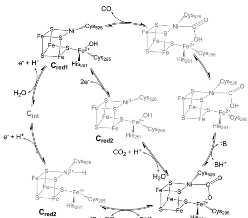
Fig. 1 Proposed catalytic cycle for CO oxidation and CO 2 reduction at the C-cluster of CODH showing two different hypothesized structures for C red2 . Amino acid numbering is from CODH II Ch . Structures in gray indicate intermediate states that are not well-characterized.
