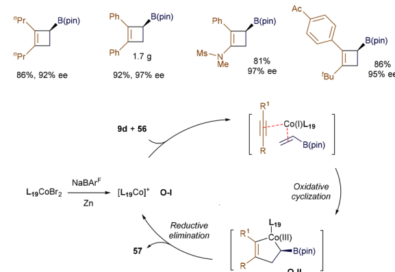
Scheme 21 Co(I)-catalyzed [2 + 2] cycloaddition.
