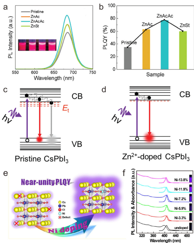
Fig. 8 (a) PL spectra of pristine and \text{Zn}^{2+} -doped \text{CsPbI}_3 NCs and their PL photographs under UV lamps. (b) PLQYs of pristine and \text{Zn}^{2+} -doped \text{CsPbI}_3 NCs. Schematic illustration of radiative and nonradiative recombination of \text{CsPbI}_3 NCs (c) before and (d) after \text{Zn}^{2+} doping. CB and VB refer to conduction band and valence band respectively. (e) Schematic illustration of \text{Ni}^{2+} doping in \text{CsPbCl}_3 NCs to achieve near-unity PLQY. (f) Absorption and PL spectra of undoped and \text{Ni}^{2+} doped \text{CsPbCl}_3 NCs. Insets show the photographs of NC solution under UV (365 nm) illumination. (a)–(d) Reproduced with permission from ref. 36. Copyright 2020, Royal Society of Chemistry (United Kingdom); (e) and (f) reproduced with permission from ref. 78. Copyright 2018, American Chemical Society.
