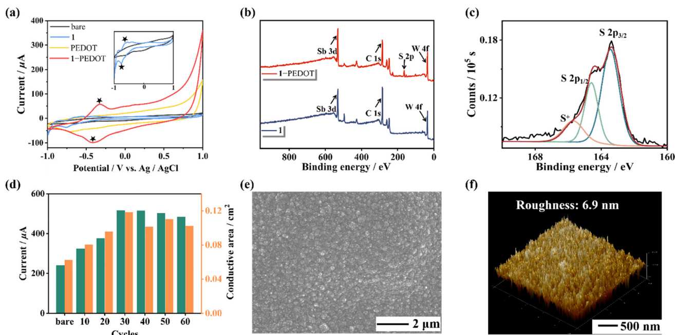
Fig. 4 (a) CV curves of bare GCE and GCEs modified using 1 , 1 -PEDOT and PEDOT in 0.2 mol \text{L}^{-1} \text{CH}_3\text{COOH}-\text{CH}_3\text{COONa} buffer solution. Inset: CV curves of bare GCE and 1 -PEDOT/GCE. (b) Comparison of XPS spectra between 1 and the 1 -PEDOT film. (c) XPS spectra of S 2p in the 1 -PEDOT film. (d) Comparison of the conductive area and DPV peak of 1 -PEDOT/GCEs with different electropolymerization cycles (0/10/20/30/40/50/60) in the Fe-PBS solution (pH = 7.4). (e and f) SEM and AFM images of the 1 -PEDOT film on the ITO substrate (30 electropolymerization cycles).
