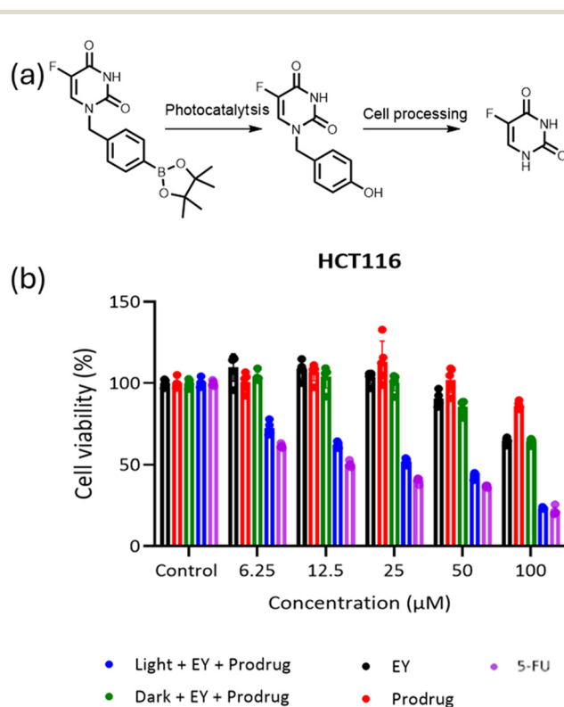
Fig. 5 The viability of HCT116 cancer cells treated with varying concentrations of the prodrug, PEG 113 - b -PAEMA + 50 -EYHEMA 1 (shortened as EY), the combination of the prodrug and PEG 113 - b -PAEMA 50 -EYHEMA 1 before and after blue light LED irradiation, and a control of just 5-FU. The cells were treated for 72 h with the indicated concentrations of the compounds. Data are presented as mean ± S.D, n = 5.
