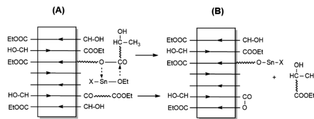
Scheme 6 Two transesterification mechanisms leading to the removal of longer chain ends.
