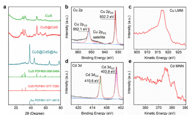
Fig. 2 (a) XRD patterns of \text{CuS} , \text{CuS}@ \text{CdS} , and \text{CuS}@ \text{CdS}@ \text{Au} NSs and their corresponding standard PDF cards. XPS spectra of (b) \text{Cu} 2p, (c) \text{Cu} LMM, (d) \text{Cd} 3d, and (e) \text{Cd} MNN in \text{CuS}@ \text{CdS}@ \text{Au} NSs.
