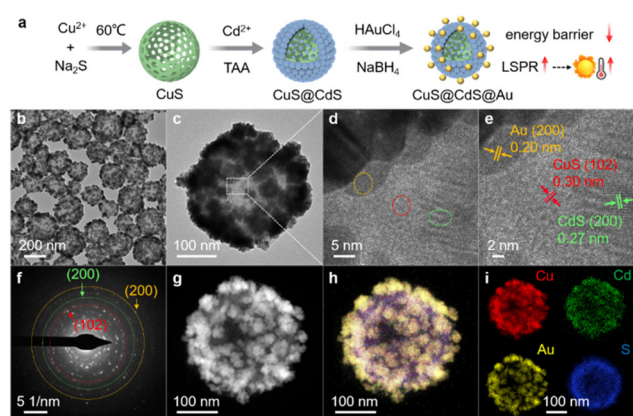
Fig. 1 (a) Schematic illustration of the synthetic process of \text{CuS}@ \text{CdS}@ \text{Au} NSs. (b and c) TEM images and (d and e) HR-TEM images of \text{CuS}@ \text{CdS}@ \text{Au} NSs. (f) SAED pattern of \text{CuS}@ \text{CdS}@ \text{Au} NSs. (g) HAADF-STEM image of \text{CuS}@ \text{CdS}@ \text{Au} NSs. (h and i) Elemental mapping images of \text{Cu} , \text{Cd} , \text{Au} , and \text{S} in \text{CuS}@ \text{CdS}@ \text{Au} NSs.
