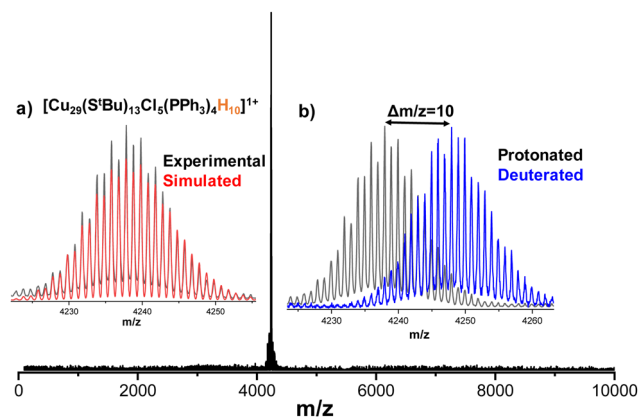
Fig. 3 Positive mode ESI MS spectrum of [\text{Cu}_{29}(\text{S}^t\text{Bu})_{13}\text{Cl}_5(\text{PPh}_3)_4\text{H}_{10}]^+ nanocluster. The peak at m/z 4237.8 corresponds to the molecular ion peak. Insets: (a) Exact matching of experimental (black trace) and simulated (red trace) isotopic distributions confirm the assigned compositions. (b) Comparison of protonated, [\text{Cu}_{29}(\text{S}^t\text{Bu})_{13}\text{Cl}_5(\text{PPh}_3)_4\text{H}_{10}]^+ , and deuterated, [\text{Cu}_{29}(\text{S}^t\text{Bu})_{13}\text{Cl}_5(\text{PPh}_3)_4\text{D}_{10}]^+ , molecular ion peaks.
