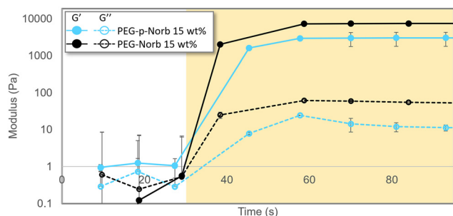
Fig. 1 Photo-rheological data of gelation for norbornene systems at 15 wt%. The shaded region indicates when the sample was being irradiated by a UV source (0.1 wt% LAP, 365 nm, 20 mW cm -2 , 250 \mu m thick). Systems reach their max storage modulus plateau within tens of seconds. For both compositions, phthalaldehyde containing systems have a decreased storage modulus. Error bars represent mean \pm SD, n = 3.
