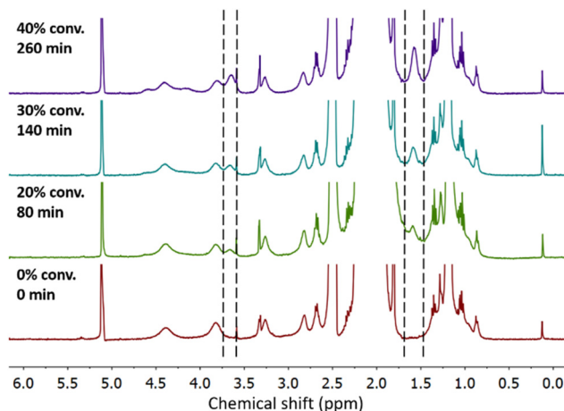
Fig. 6 Conversion of epoxides during a ring-opening reaction of GMA-EGDMA-S + with 5 equiv. of diethyl sulfide in AcOH/acetone 1:1, as analyzed by ^1\text{H} NMR spectroscopy in acetone- d_6 . Conversion was calculated utilizing 1,3,5-trioxane as an internal standard. Its singlet peak can be seen at 5.1 ppm.
