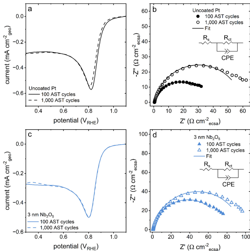
Fig. 7 (a and c) Linear sweep voltammometry plots recorded at a scan rate of 10 mV s -1 in an O 2 (g) saturated electrolyte for the pristine and coated Pt samples after performing (solid line) 100 cycles and (dashed line) 1000 cycles of the AST. (b and d) Nyquist plots recorded at 0.9 V RHE in an O 2 saturated electrolyte with fits (solid lines) corresponding to the circuit displayed in the inset also obtained after performing (solid symbols) 100 cycles and (hollow symbols) 1000 cycles of the AST. The colours of the traces correspond to the thickness of the Nb 2 O 5 films where black is uncoated, pristine Pt and blue is Pt with a 3 nm thick coating of Nb 2 O 5 .
