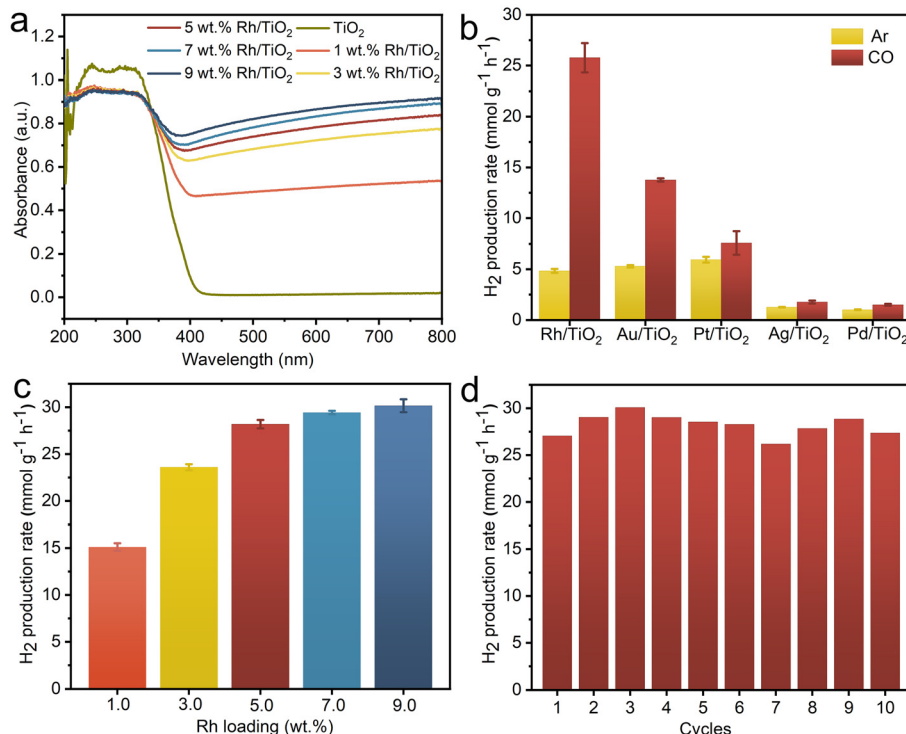
Fig. 3 (a) Absorption spectra for \text{TiO}_2 and x wt.% \text{Rh/TiO}_2 ; (b) triphase photocatalytic \text{H}_2 production rate for 5 wt.% \text{M/TiO}_2 ( \text{M} = \text{Rh}, \text{Au}, \text{Ag}, \text{Pt}, \text{Pd} ) in Ar or CO atmosphere; (c) photocatalytic \text{H}_2 production rate as a function of the loading amount of Rh in \text{Rh/TiO}_2 ; (d) cycling tests for \text{Rh/TiO}_2 . Reaction conditions: gas phase = 0.2 MPa of CO, liquid phase = 10 mL of \text{H}_2\text{O} , solid phase = 2 mg of photocatalyst immobilized on GDL (4 cm in diameter), light source = 365 nm LED ( 300 \text{ mW cm}^{-2} ). Error bars represent the standard deviation from at least three independent measurements.
