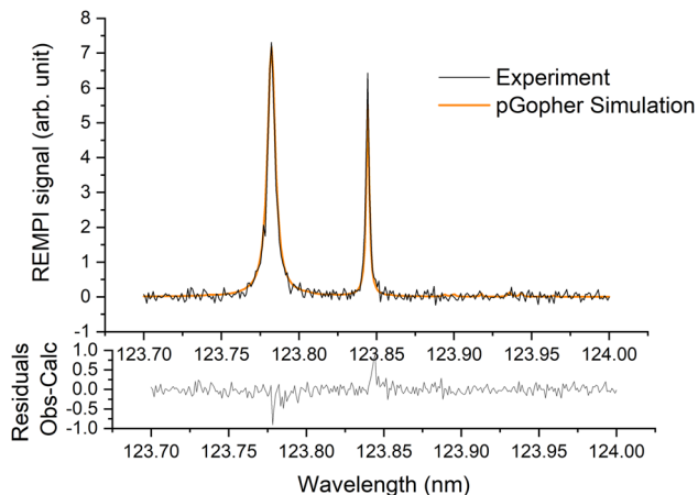
Fig. 2 Experimental (in black) and simulated (in orange) (2 + 1) REMPI spectra of the C^1B_1, v = 0 \leftarrow X^1A_1, v = 0 transition of HDO in the supersonic beam. See Yang et al. 21 for more details.
