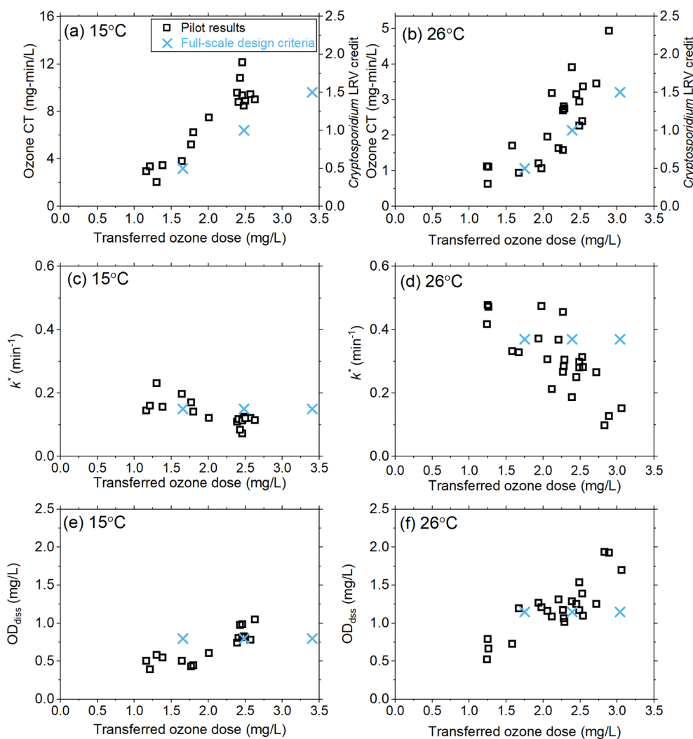
Fig. 6 Comparing pilot-scale results of this study to the initial full-scale design criteria at low (15 °C, left panels) and high (26 °C, right panels) design temperatures in terms of the effect of transferred ozone doses on (a and b) ozone CT (left y-axis) and LRV targets (right y-axis), (c and d) k^* , and (e and f) \text{OD}_{\text{diss}} .
