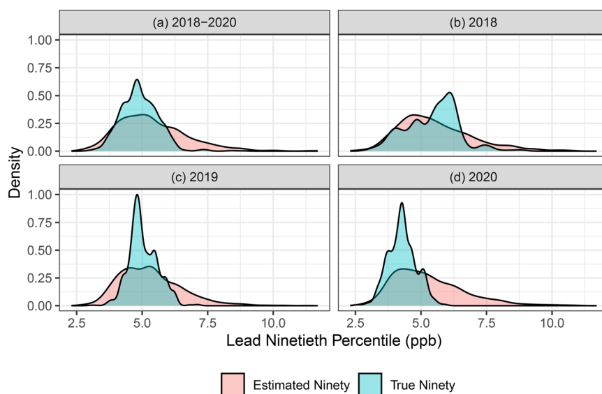
Fig. 1 Distribution of 'true' and 'estimated' L5 ninetyeth percentile results for DC Water from 1000 simulations for each of the four datasets: (a) simulated LCR sampling rounds were generated by randomly selecting from all paired L1 and L5 samples from 2018–2020, (b) sample rounds were generated by using paired samples from the two 2018 LCR sample rounds, (c) sample rounds were generated by using paired samples from the two 2019 sample rounds, and (d) sample rounds were generated by using paired samples from the two 2020 sample rounds.
