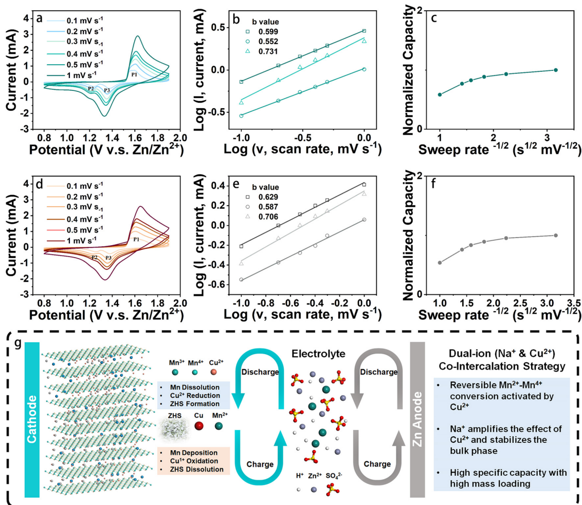
Fig. 4 (a) and (d) CV curves with scan rates ranging from 0.1 to 1 \text{ mV s}^{-1} , (b), (e) diffusion-capacitive control contribution, and (c) and (f) the relationship between normalized capacity and sweep rate of NCMO and NMO, respectively. (g) Schematic diagram illustrating the charge and discharge process of NCMO cathodes in ZIBs.
