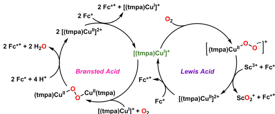
Fig. 5 Proposed catalytic cycles for the reduction of dioxygen by [\text{Cu}^{\text{II}}(\text{tmpa})(\text{CH}_3\text{CN})](\text{HClO}_4)_2 , where (\text{tmpa}) = \text{tris}(2\text{-pyridylmethyl})\text{amine} , in the presence of Brønsted Acids (left) and Lewis Acids (right). The mechanistic differences between the two cycles result in a quantitative shift in selectivity from water (Brønsted) to hydrogen peroxide (Lewis). Adapted from ref. 47 and 48.
