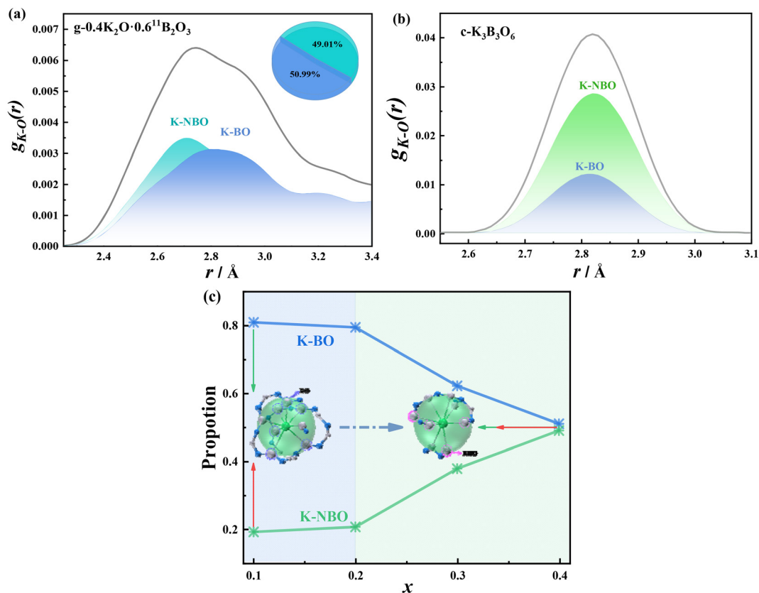
Fig. 6 (a) The distribution of K–BO and K–NBO interactions in the first coordination layer of the K–O interaction in 0.40K_2O \cdot 0.60^{11}B_2O_3 glass. The pie chart on the right shows the percentages of each atom-pair interaction. (b) The distribution of K–BO and K–NBO interactions in the first coordination layer of the K–O interaction in the K_3B_3O_6 crystal. (c) Changes in the relative contents of K–BO and K–NBO interactions in xK_2O \cdot (1-x)^{11}B_2O_3 ( 0.1 \leq x \leq 0.4 ) glass.
