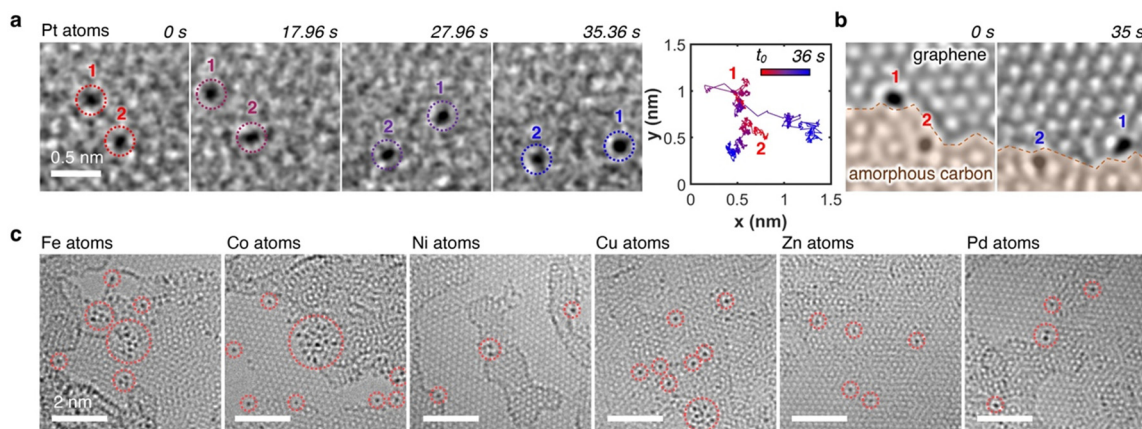
Fig. 3 Released single metal atoms. (a) Time-dependent sequence of two Pt atoms. The coloration of the metal atoms corresponds to the time stamp from the respective trajectories. (b) Images of stacked sequence (25 frames corresponding to 1 s exposure time), highlighting the location of each atom. Atom 1 is located on the graphene monolayer at the edge of an amorphous carbon layer; atom 2 is embedded within the amorphous carbon layer. (c) Overview images of remaining single metal atoms (Fe, Co, Ni, Cu, Zn, Pd) released by the e-beam.
