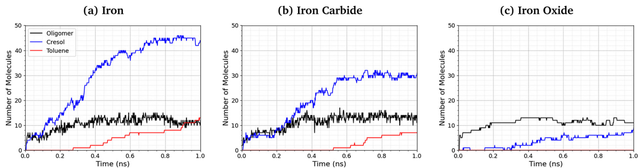
Fig. 9 Comparison of oligomer, toluene, and cresol quantities at 500 K and 3 GPa for the (a) \alpha -Fe(110), (b) Fe 3 C(010), and (c) Fe 3 O 4 (001) systems.
