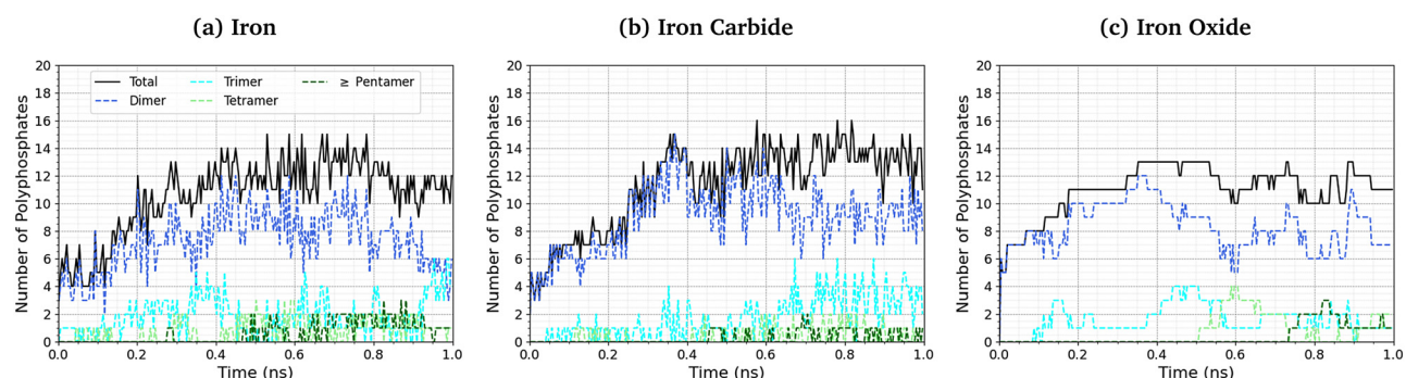
Fig. 10 Change in the number of polyphosphate chains with sliding time at 500 K and 3 GPa for (a) \alpha -Fe(110), (b) Fe 3 C(010) and (c) Fe 3 O 4 (100) systems.
