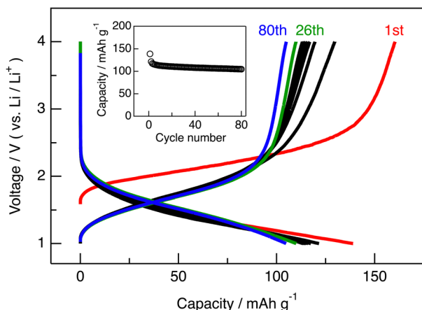
Fig. 3 Charge/discharge curves for \text{Li}_2\text{NbHO}_2 electrode between 1.0 and 4.0 V (vs. \text{Li}/\text{Li}^+ ) at a rate of \text{C}/10 ( = 38.3 \text{ mA g}^{-1} ) at 25^\circ\text{C} . Inset: Discharge capacity retention upon cycling up to 80 cycles. Li metal foil was used as the counter electrode, and 1 M \text{LiPF}_6 dissolved in a 1 : 1 v/v mixture of ethylene carbonate/diethyl carbonate (EC/DEC; Kishida Chemical) was employed as the electrolyte. Working electrode was formulated with 83 wt% active materials, 10 wt% acetylene black, and 7 wt% polytetrafluoroethylene (PTFE).
