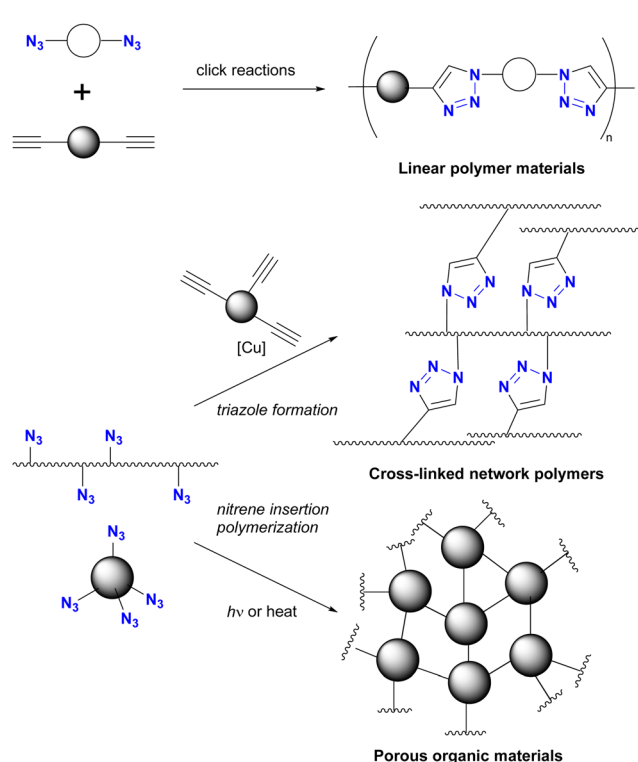
Fig. 3 The general approach to crosslinked polymers by multiple CuAAC.
