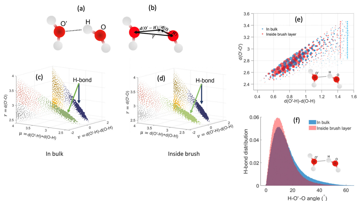
Fig. 26 (a) Schematic of the water–water hydrogen bond formation. We identify the hydrogen atom (H), the donor oxygen atom (O), and the acceptor oxygen atom (O'). (b) Identification of the distances \nu = d(\text{O}-\text{H}) - d(\text{O}'-\text{H}) , \mu = d(\text{O}-\text{H}) + d(\text{O}'-\text{H}) , and r = d(\text{O}'-\text{O}) . (c) and (d) The distribution of ( \nu , \mu , and r ) characterizing the water–water hydrogen bonding for water in (c) bulk and (d) inside the PMETAC PE brush layer. Clusters representing different interactions have been colored differently with the clusters representing water–water hydrogen bonding identified. (e) Variation of ( \nu , r ) characterizing the water–water hydrogen bonding for water in bulk and inside PMETAC PE brush layer with the average location (in \nu ) of the edge of hydrogen bond cluster identified for both the cases. (f) Normalized distribution of the water–water HBs (for water molecules in bulk and inside the brush layer) as functions of the H–O'–O angles. All the parts of the figure have been reproduced from Pial, T. H.; Das, S., Machine learning enabled quantification of the hydrogen bonds inside the polyelectrolyte brush layer probed using all-atom molecular dynamics simulations, Soft Matter , 2022, 18 (47), 8945–8951. Copyright (2022) Royal Society of Chemistry (UK).
