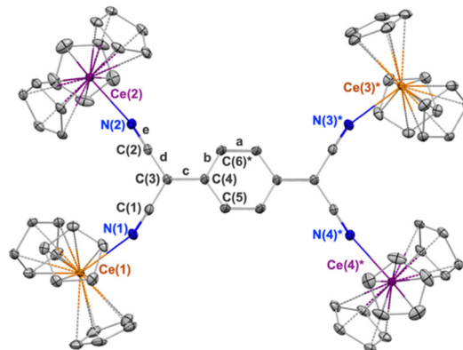
Fig. 1 Thermal ellipsoid plot of 1 shown at the 30% probability level. \text{Ce}^{\text{III}} centers are shown in orange and \text{Ce}^{\text{IV}} in purple color. The * indicates atoms at equivalent position ( -x, 1-y, 1-z ). Hydrogen atoms and co-crystallized toluene molecules are omitted for clarity.
