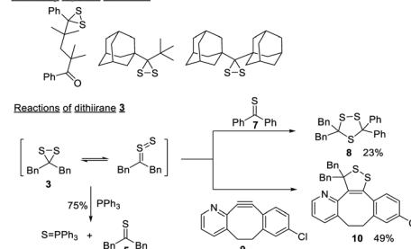
Scheme 4 The structures of reported dithiiranes and dithiirane 3 's reactions.
