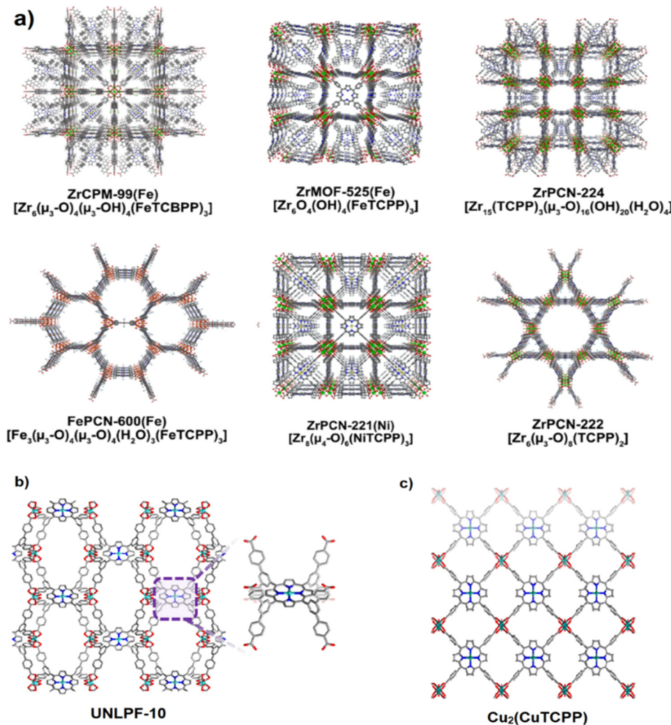
Fig. 17 Porphyrin-based MOFs can be transformed into PC functional materials. Color scheme: Zr (green); Fe (orange); Ni (yellow) O (red); N (blue); C (a). Structure of UNLFP-10 featuring In-porphyrin sites for the photocatalytic oxidation of thioanisole (b). Structure of \text{Cu}_2(\text{CuTCPP}) featuring \text{Cu}_2 nodes and Cu-porphyrin sites for the electrochemical reduction of \text{CO}_2 to formate and acetate (c). Reproduced from ref. 140 and 141 with permission with Elsevier.
