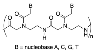
Fig. 1 General structure of a portion of the polyamide backbone of the peptide nucleic acid: a dimer.
