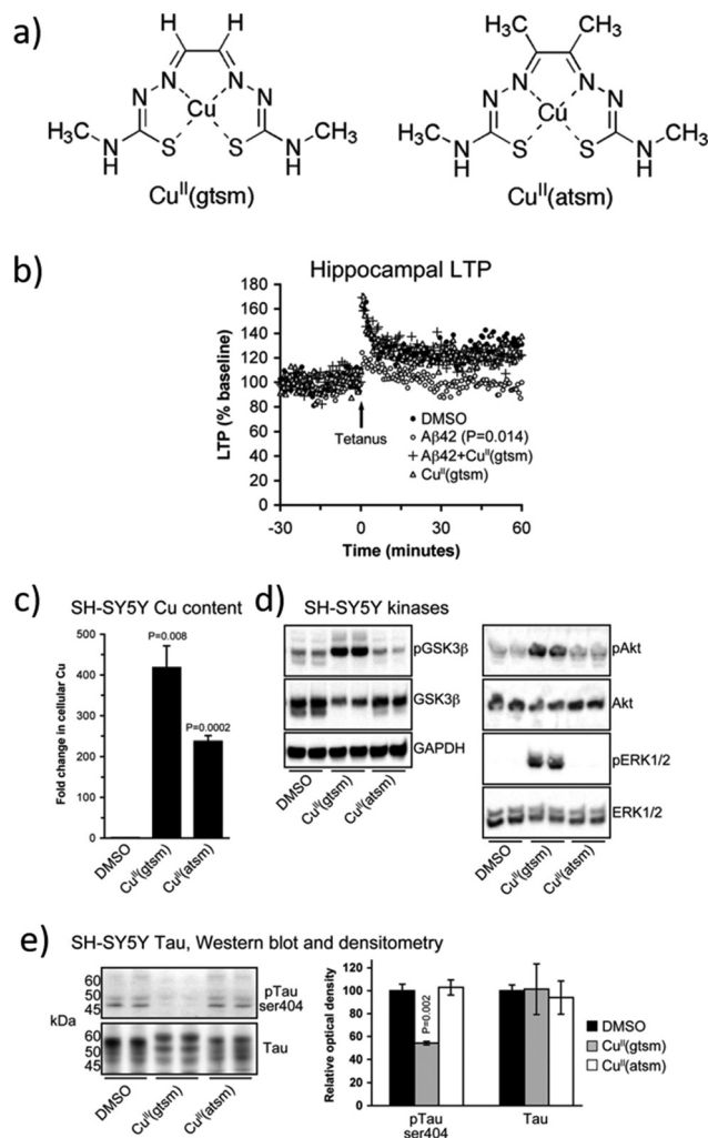
Fig. 5 (a) Structures of [Cu II (gtms)] and the control [Cu II (atms)]. (b) Whereas Aβ 42 inhibits the hippocampal long-term potentiation (LTP) by 28%, this is prevented when treated with [Cu II (gtms)]. (c) In vitro , [Cu II (gtms)] increases the cellular levels of Cu. (d) Western blot analyses show that [Cu II (gtms)] induces the phosphorylation of kinases GSK3β, Akt, and ERK1/2. (e) [Cu II (gtms)] inhibits tau phosphorylation at ser404 without affecting the abundance of total tau. Adapted from Ref. 68. Reproduced with permission.
