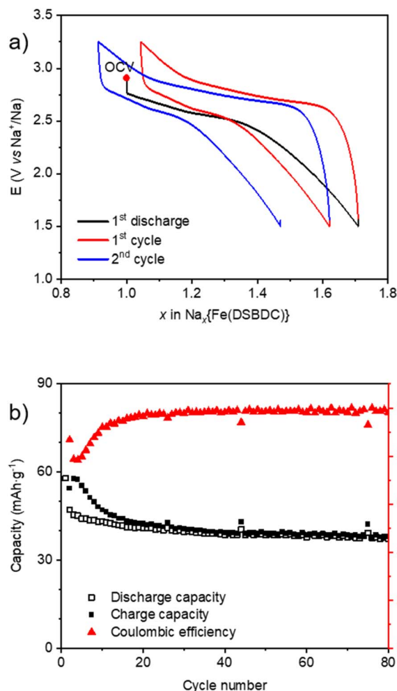
Fig. 8 Electrochemical behaviour of Na{Fe(DSBDC)} in a half-cell vs. Na cycled in the voltage range of 1.5–3.25 V vs. Na + /Na (1 e - exchanged per Fe in 10 h). (a) Potential vs. a number of inserted/extracted Na + in the first two cycles. (b) Corresponding capacity retention and coulombic efficiency curves upon long-term cycling.
