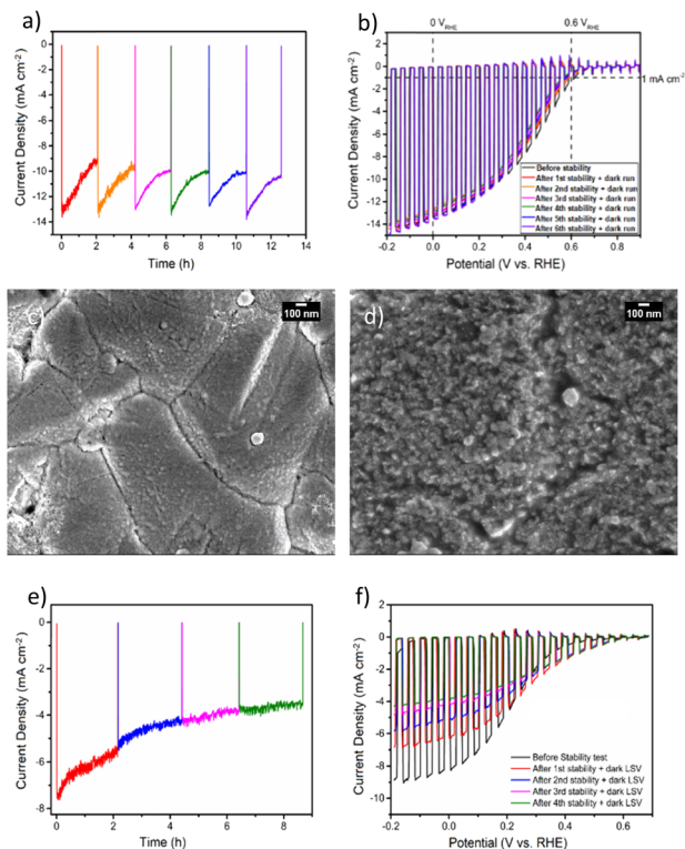
Fig. 4 (a) Current–time curve of CZTS/CdS/ITO/Pt in 1 M \text{K}_2\text{HPO}_4/\text{KH}_2\text{PO}_4 (pH 7) under solar simulated AM 1.5G light irradiation at an applied bias of 0 \text{ V}_{\text{RHE}} . The stability test is conducted at 2 h intervals with 3 recovery dark LSV sweeps at every interval. (b) Corresponding chopped LSV before the stability test and after each recovery dark LSV sweep. Scanning electron microscopy (SEM) of CZTS/CdS/ITO/Pt after 12 h stability test (c) with recovery dark LSV (d) without recovery dark LSV sweeps. (e) Stability test and (f) corresponding LSV for the photocathode without ITO (CZTS/CdS/Pt).
