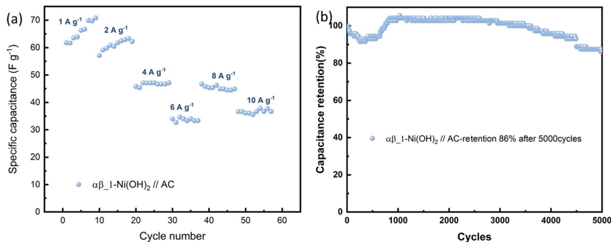
Fig. 11 (a) The specific capacitance evolution under various current densities of \alpha\beta_1 - \text{Ni(OH)}_2 // \text{AC} . (b) Cycling performance at 100 \text{ mA cm}^{-2} for 5000 cycles.
