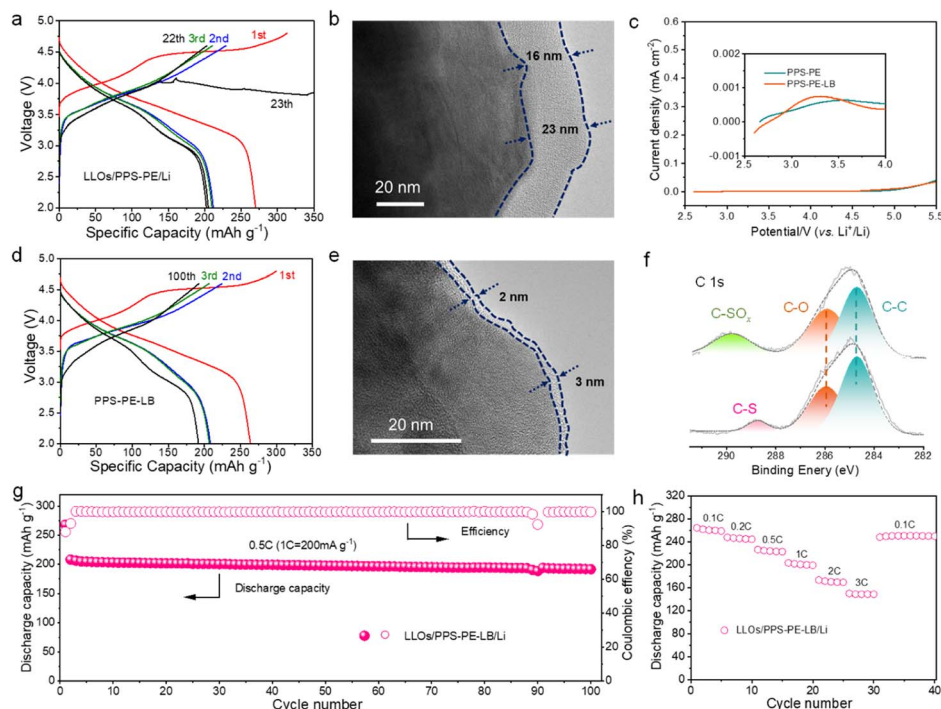
Fig. 4 (a) The charge/discharge curves of the LLOs/PPS-PE/Li batteries with current densities of 0.1C and 0.5C ( 1C = 200 \text{ mA g}^{-1} ). (b) The CEI on the surface of the cathode in LLOs/PPS-PE/Li batteries after cycling. (c) The linear sweep voltammetry of PPS-PE and PPS-PE-LB. (d) The charge/discharge curves of the LLOs/PPS-PE-LB/Li batteries with two current densities. (e) The CEI on the surface of the cathode in LLOs/PPS-PE-LB/Li batteries after cycling. (f) The XPS spectra of the PPS-PE film on the cathode side before and after the cycling of the battery. (g) The cycling stability of the LLOs/PPS-PE-LB/Li battery at 0.5C in the voltage range of 2.0–4.6 V. (h) The rate performances of the LLOs/PPS-PE-LB/Li battery.
