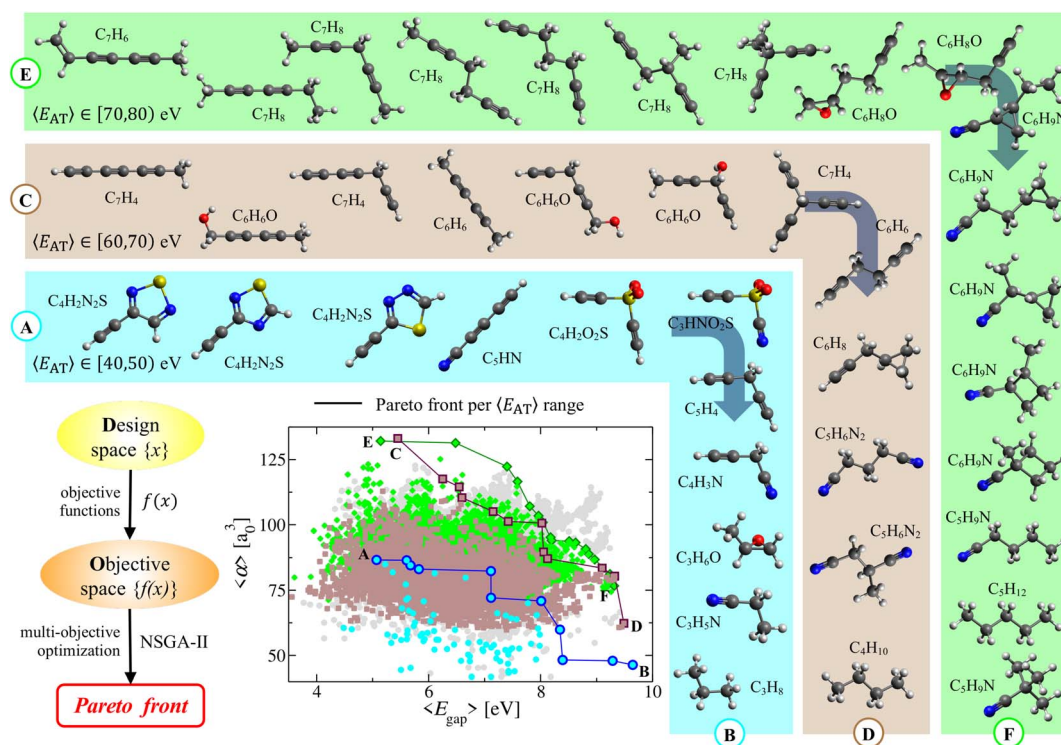
Fig. 4 Multi-property optimization: Pareto front analysis in molecular property space. Pareto (multi-property) optimization was performed on the thermally-averaged (\langle E_{\text{AT}} \rangle, \langle E_{\text{gap}} \rangle, \langle \alpha \rangle) -manifold of molecular property space ( T = 300 K) to identify molecules with simultaneously optimal \langle \alpha \rangle and \langle E_{\text{gap}} \rangle values. Depicted is a correlation plot between \langle \alpha \rangle and \langle E_{\text{gap}} \rangle , with each point colored according to the corresponding \langle E_{\text{AT}} \rangle range (cyan: \langle E_{\text{AT}} \rangle \in [40,50] eV; tan: \langle E_{\text{AT}} \rangle \in [60,70] eV; light green: \langle E_{\text{AT}} \rangle \in [70,80] eV; gray points in the background correspond to values outside these \langle E_{\text{AT}} \rangle windows. Optimal Pareto fronts corresponding to each of these \langle E_{\text{AT}} \rangle windows are provided as highlighted points (connected via solid lines) in the correlation plot; see Sec. 2 for a more detailed description of the optimization procedure. Also depicted are the QM7-X molecules located along each of these Pareto fronts (colored insets), which correspond to non-trivial paths through CCS defined by small directed structural/compositional changes that yield simultaneously optimal values for these properties.
