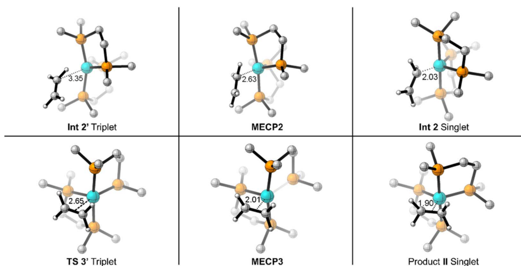
Fig. 3 3D depiction of M06-L optimized geometries for reaction between (DMPE) 2 Fe and ethylene with key bond/coordination distances (in Å).
