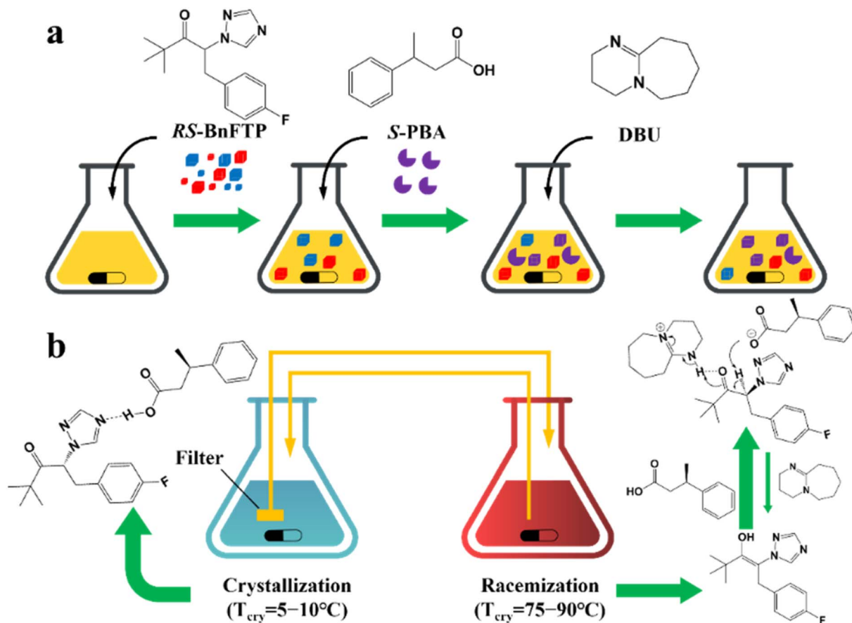
Fig. 13 (a) Schematic representation of the CoISD process and (b) the CoISD mechanism that occurred in a two-vessel setup with the cocrystal in suspension. 55,239 RS-BnFTP, PBA and DBU represent the racemic mixture, chiral coformer and racemizing agent, respectively.
