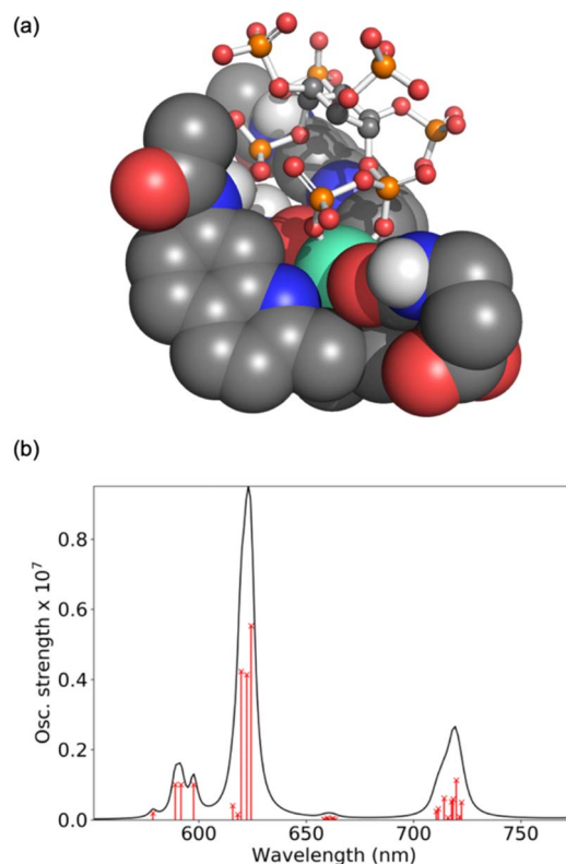
Fig. 3 Computational analysis of 5-PP-InsP 5 binding to [Eu.3] 3+ : (a) DFT optimised geometry of the bidentate binding mode and (b) ab initio luminescence spectrum from 5 D 0 showing the individual microstates of the 7 F term as red crosses on lines proportional to their oscillator strength.
