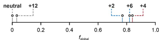
Fig. 4 Global ring current fraction, f_{\text{global}} , of c\text{-P6}\cdot\text{T6}^Q ( Q = 0, +2, +4, +6 and +12 ), calculated using (//B)_{\text{global}} and (//B)_{\text{local}} values from the MCL model using experimental NMR chemical shifts.
