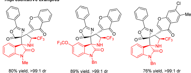
Scheme 7 TBAB-catalyzed highly diastereoselective [3+2] cycloaddition of ketimines to access spirooxindoles.
