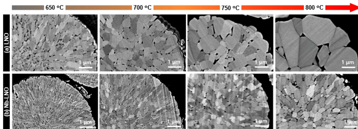
Fig. 9 Cross-sectional SEM images of (a) as-prepared LNO and (b) Nb-LNO calcined at 650 – 800^{\circ}\text{C} . Adapted from ref. 115. Copyright 2023, Wiley-VCH GmbH.
