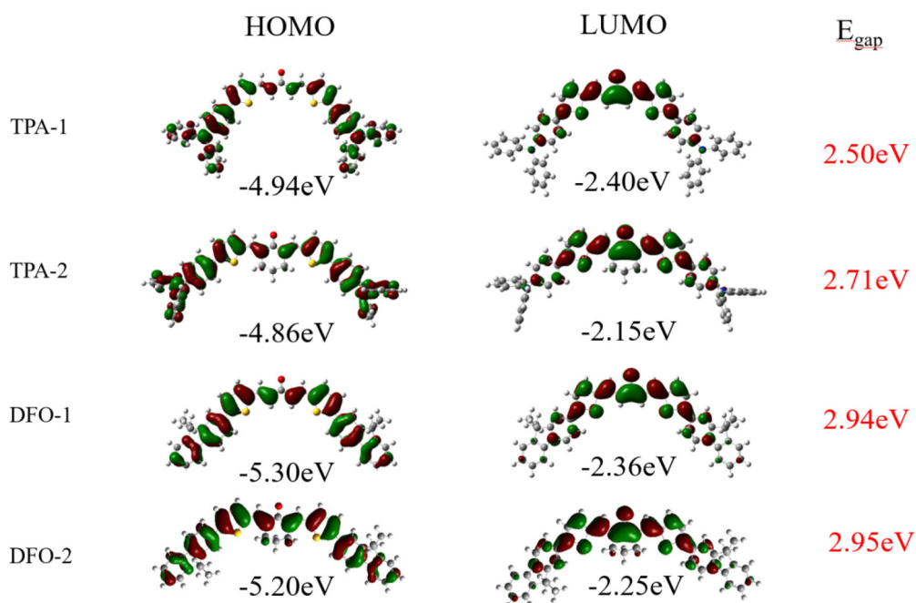
Fig. 2 HOMOs and LUMOs of the chalcones.
