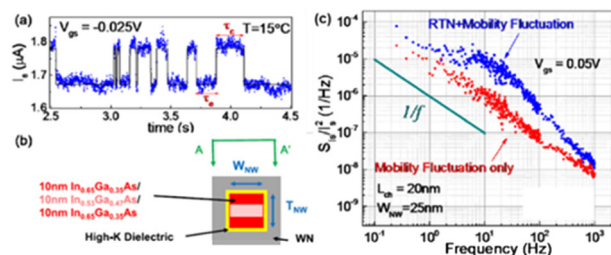
Fig. 20 (a) RTN at V_{\text{DS}} = 50 \text{ mV} for InGaAs NW MOSFET with geometry illustrated schematically in (b). The gate dielectric of the device in (a) is 0.5 nm \text{Al}_2\text{O}_3/4.0 \text{ nm} \text{LaAlO}_3 . (c) Normalized noise power spectral density vs. frequency for two InGaAs NW MOSFETs with 3.5 nm \text{Al}_2\text{O}_3 dielectrics: one showing RTN and the other showing LF noise. Adapted from ref. 67 with permission. Copyright 2015 Institute of Electrical and Electronics Engineers.
