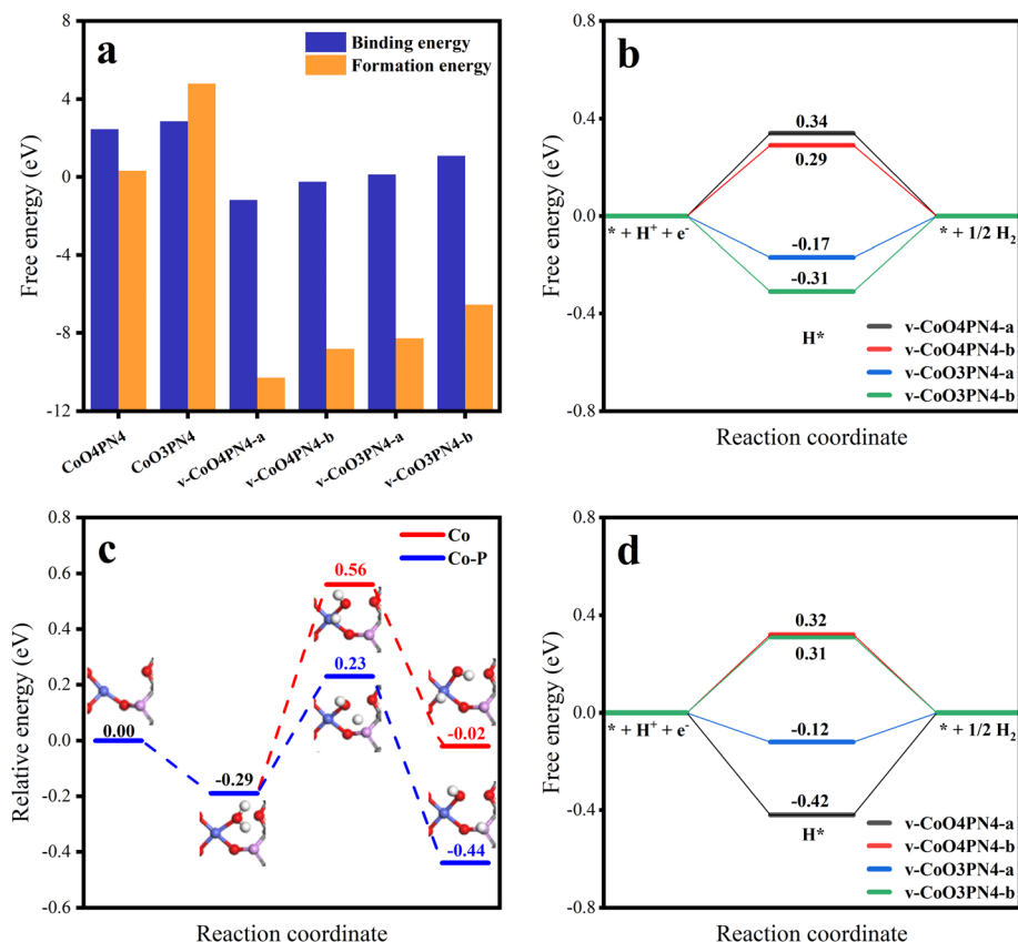
Fig. 6 (a) Binding energies and formation energies of CoO4PN4, CoO3PN4, v-CoO4PN4-a, v-CoO4PN4-b, v-CoO3PN4-a, and v-CoO3PN4-b. (b) H adsorption free energy at Co sites in v-CoO4PN4-a, v-CoO4PN4-b, v-CoO3PN4-a, and v-CoO3PN4-b. (c) Relative free energy of water splitting reaction pathway on Co site and Co-P cooperation on v-CoO3PN4. (d) H adsorption free energy at P sites in v-CoO4PN4-a, v-CoO4PN4-b, v-CoO3PN4-a, and v-CoO3PN4-b.
