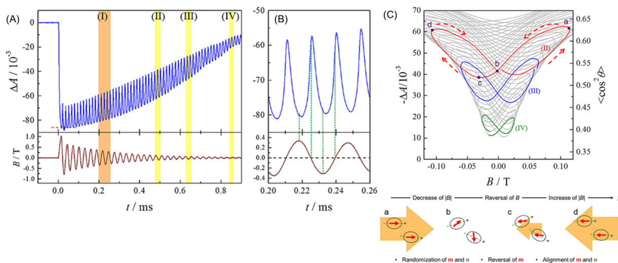
Fig. 15 (A) Typical waveform of absorbance change of MNP suspension (upper) and DOMF (bottom). (B) Enlargement of region I in (A). (C) Plots of \Delta A ( \langle \cos^2 \theta \rangle ) against B. The colored lines show the region highlighted in (A). Temporal direction of the curve is depicted by dashed arrows. The bottom figure illustrates the speculated behavior of magnetic moment (red arrows) and the easy axis (green dashed line) during the half period of field oscillation. Reprinted with permission from ref. 230. Copyright © 2019, American Institute of Physics.
