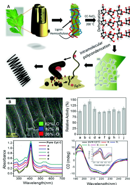
Fig. 9 Schematic depictions of (A) a plausible mechanism of the sequential growth of TLFCHs from Parthenium biomass during a solvo-thermal process in the presence of a DES (CC : FeCl 3 , 1 : 2 mol ratio) (B) Cyt C immobilized on TLECH and showing activity and stability results (ref. 50).
