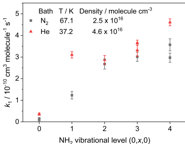
Fig. 4 Rate coefficients for the removal of \text{NH}_2 ( \nu = 0-4 ) with \text{CH}_3\text{CHO} . Grey squares; T = 67.1 K, [\text{N}_2] = 2.5 \times 10^{16} molecules per \text{cm}^3 . Red triangles; T = 37.2 K, [\text{He}] = 4.6 \times 10^{16} molecules per \text{cm}^3 .
